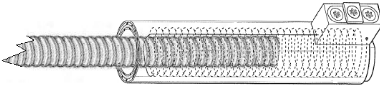
Slide-over style cylinder sensor
